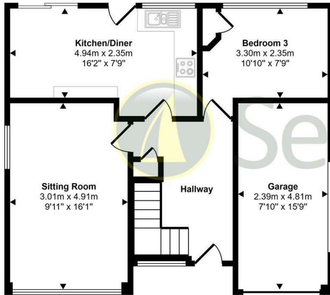
Ground Floor Approx 59 sq m / 639 sq ft
